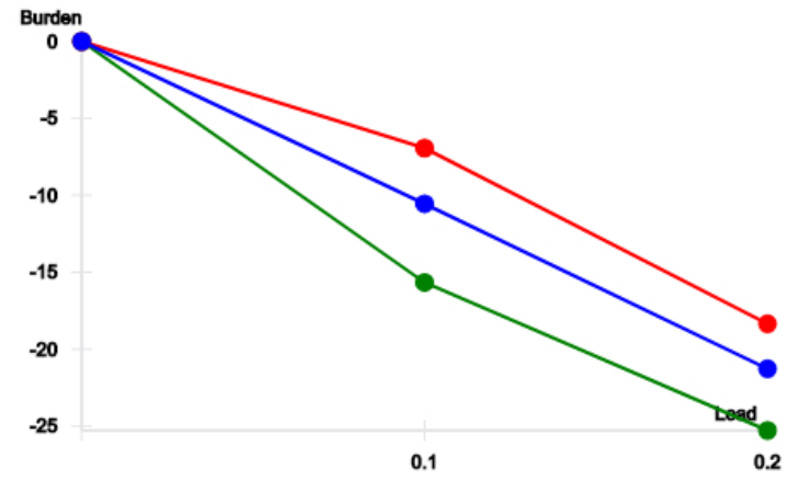
Parallelogram
